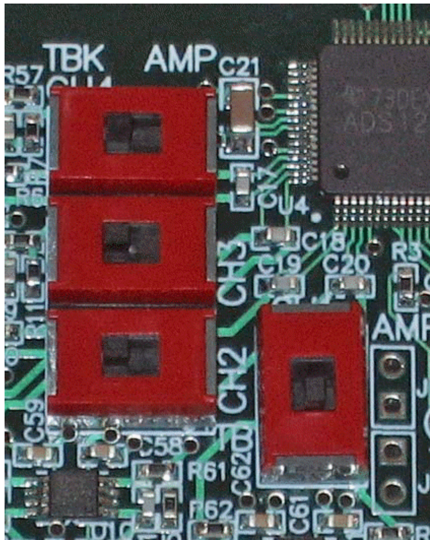
Figure 7. Amplifier Selection Switches
