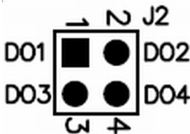
Figure 2. Connector J2
