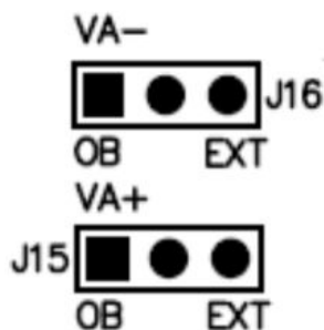
Figure 3. Connectors J15, J16
